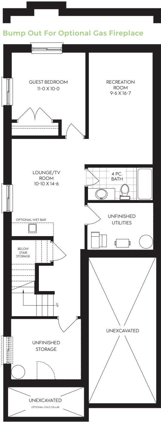
Finished Basement | +719 sq.ft.
