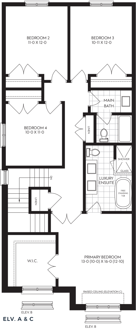
1 | Alt. Second Floor | 1213 sq.ft. 4 Bed Layout With Luxury Ensuite
