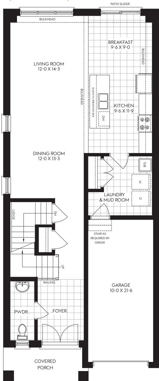
Main Floor
