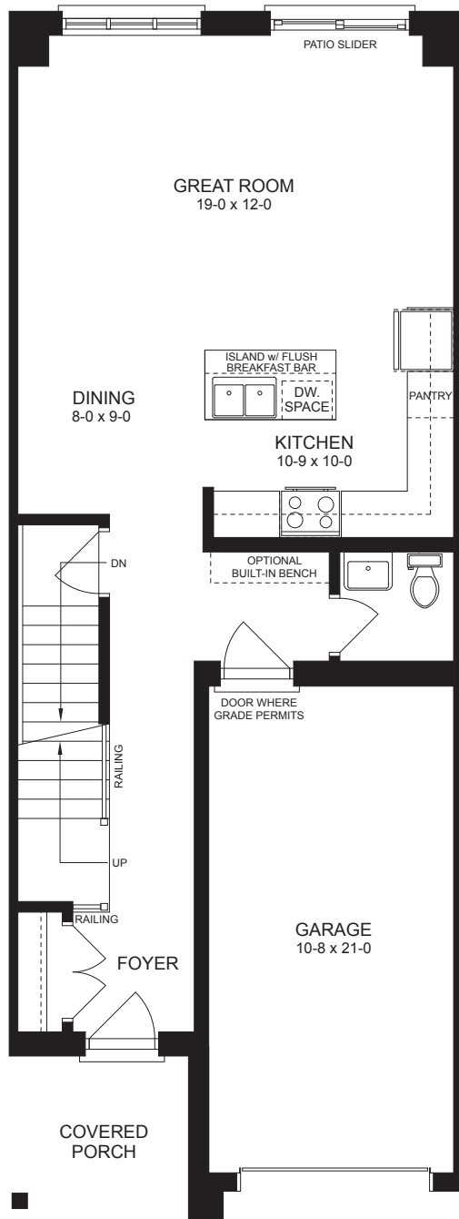
Main Floor
