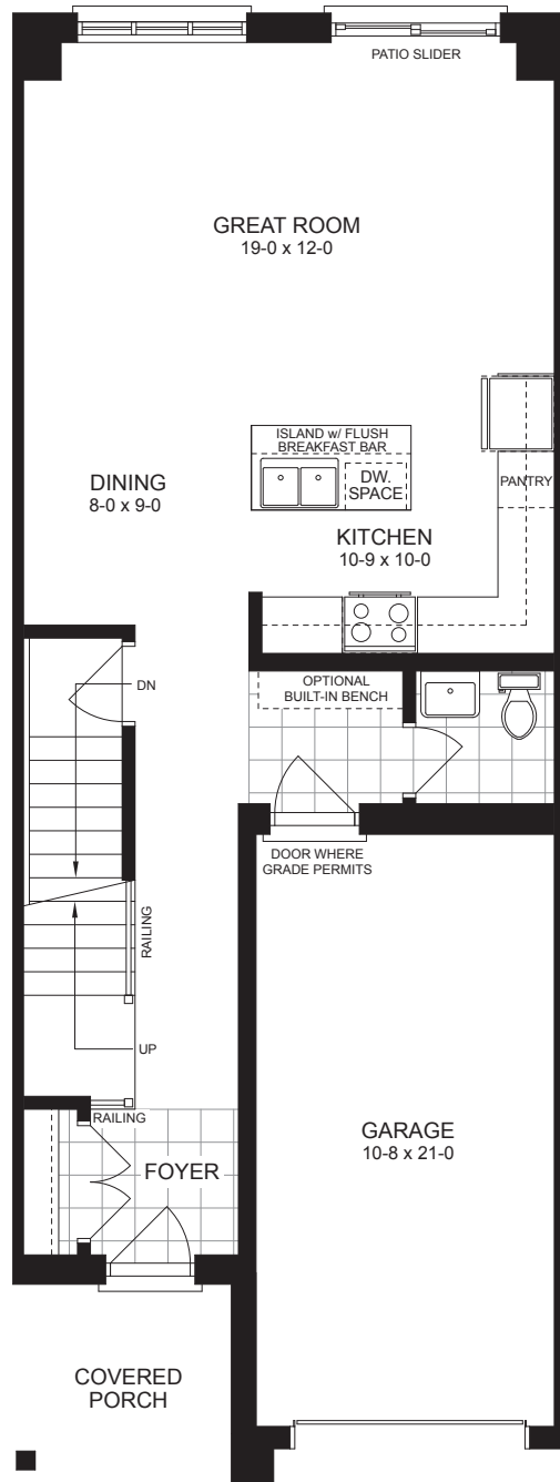
Main Floor
