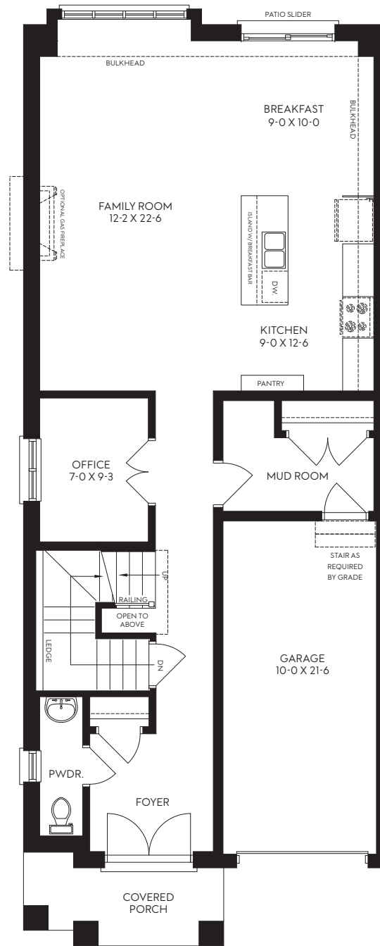
Alt. Main Floor
