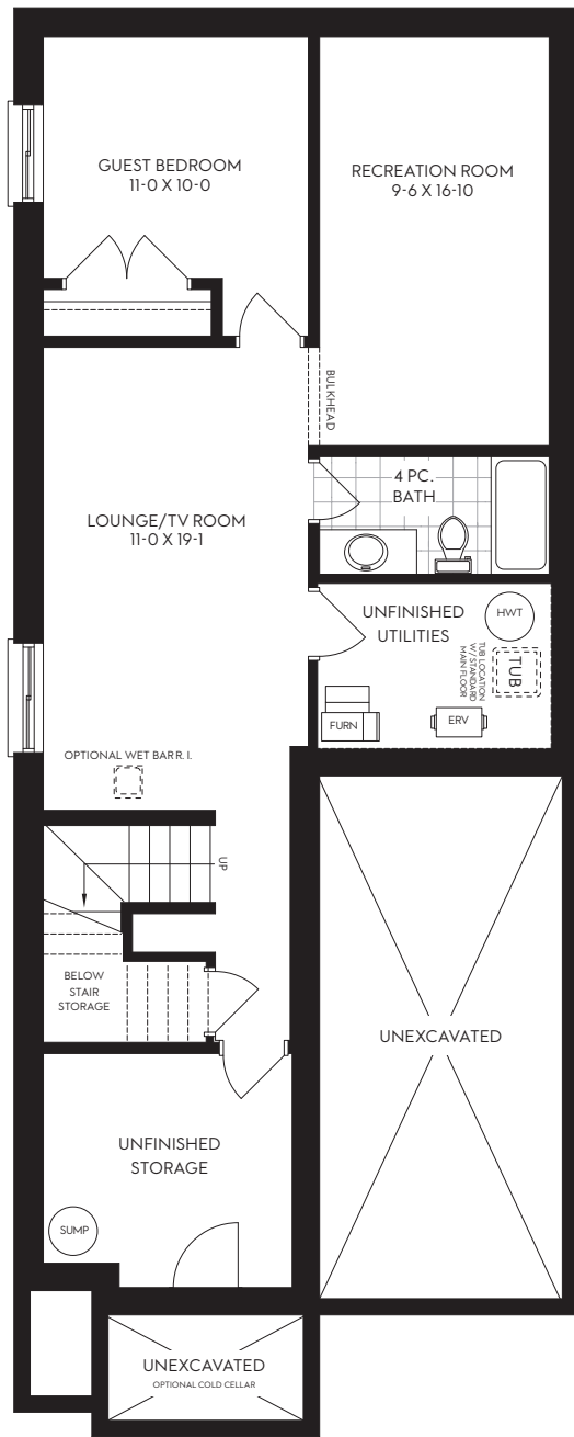
Finished Basement | +754 sq.ft.
